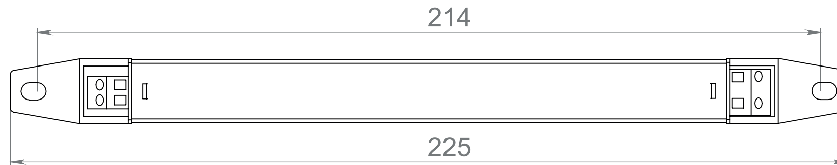
CSVT 36W-350mA-E-08
