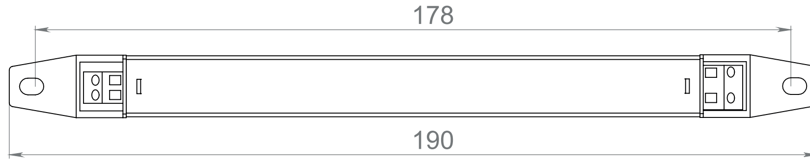
CSVT 18W-350mA-E-08
