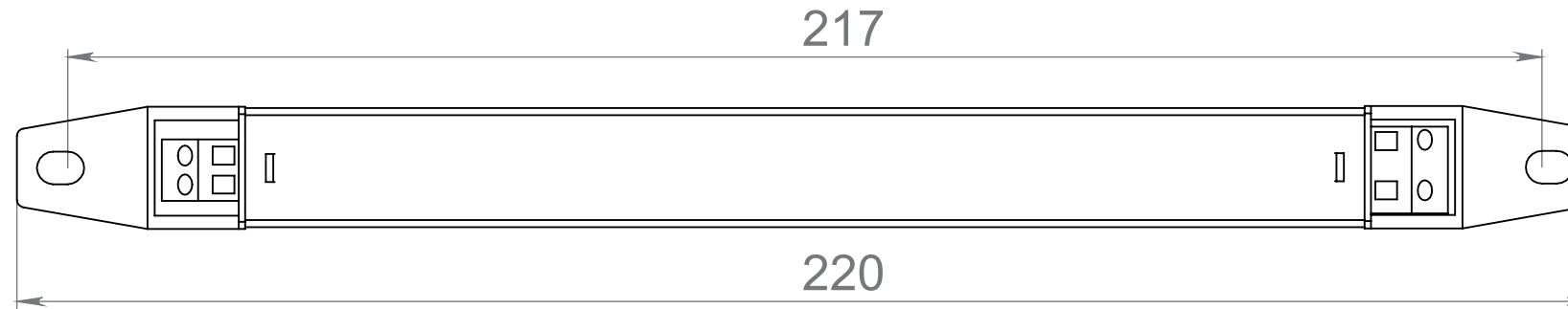
CSVT 32W-300mA-E-08
